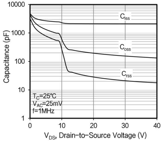
Figure 7. Capacitance Characteristics
