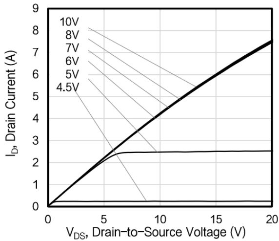
Figure 1. On-Region Characteristics
