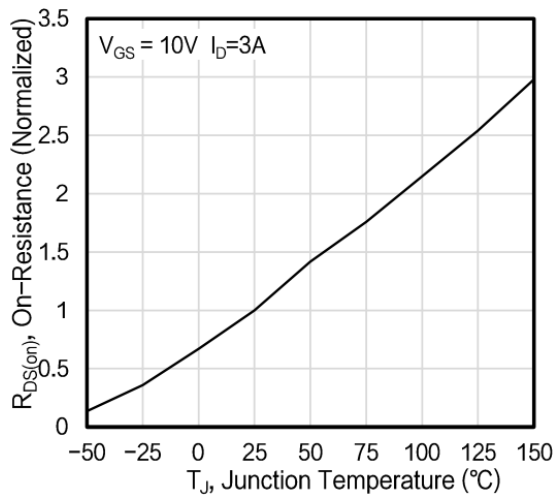
Figure 5. Normalized R_{DS(on)} vs. Temperature
