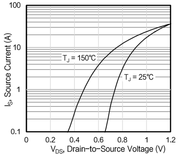
Figure 4. Typical Body Diode Transfer Characteristics
